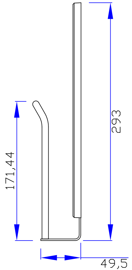
(Side View)
