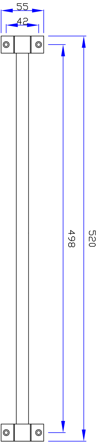
(FRONT VIEW)
