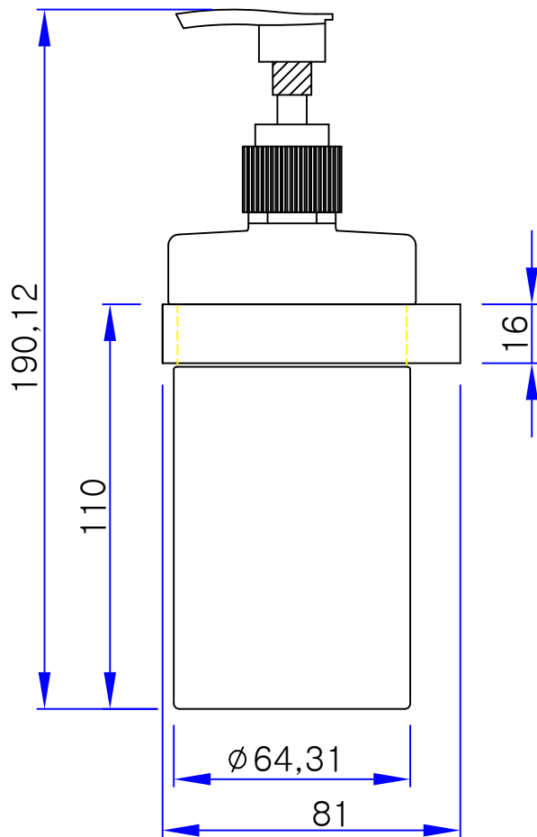
(Front View)
