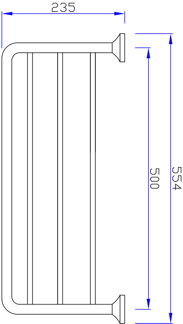
(Top View)
