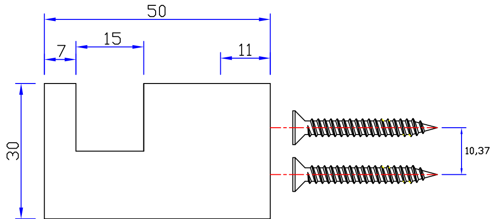
(Side View)
