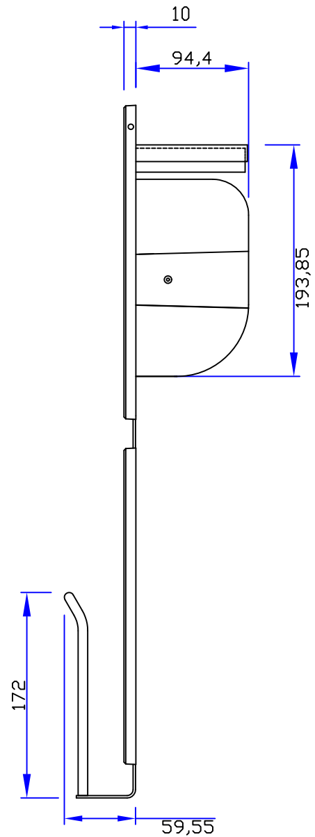
(Side View)
