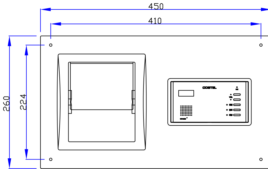
(Front View)
