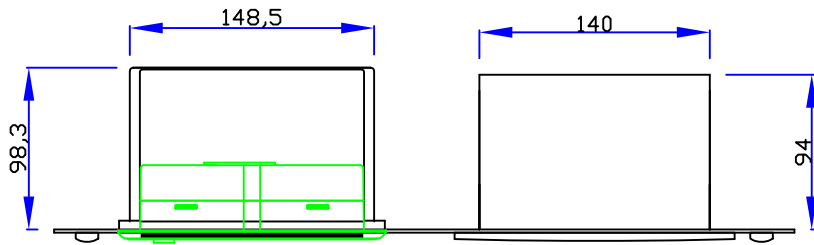
(Top View)
