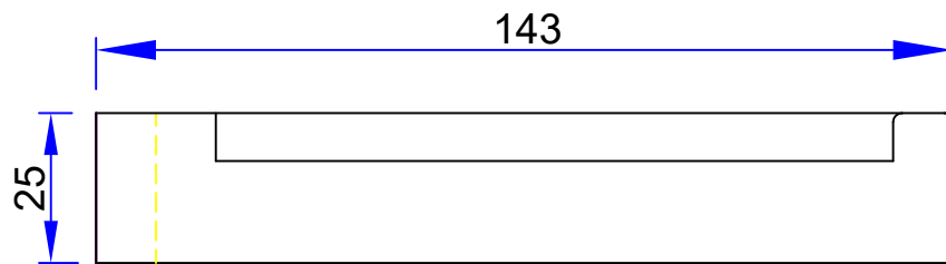
(Front View)
