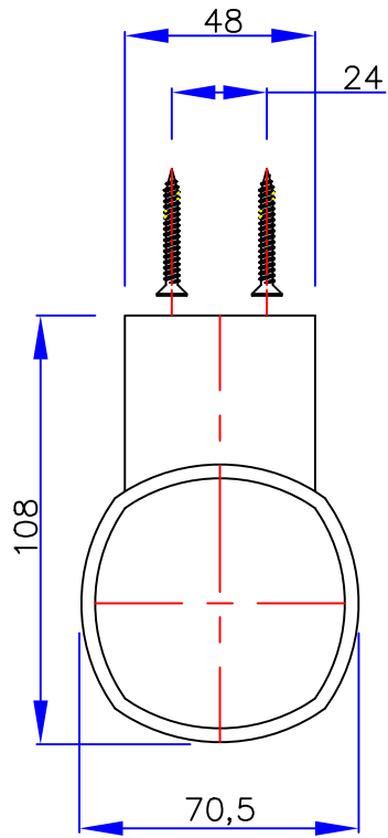
(Top View)
