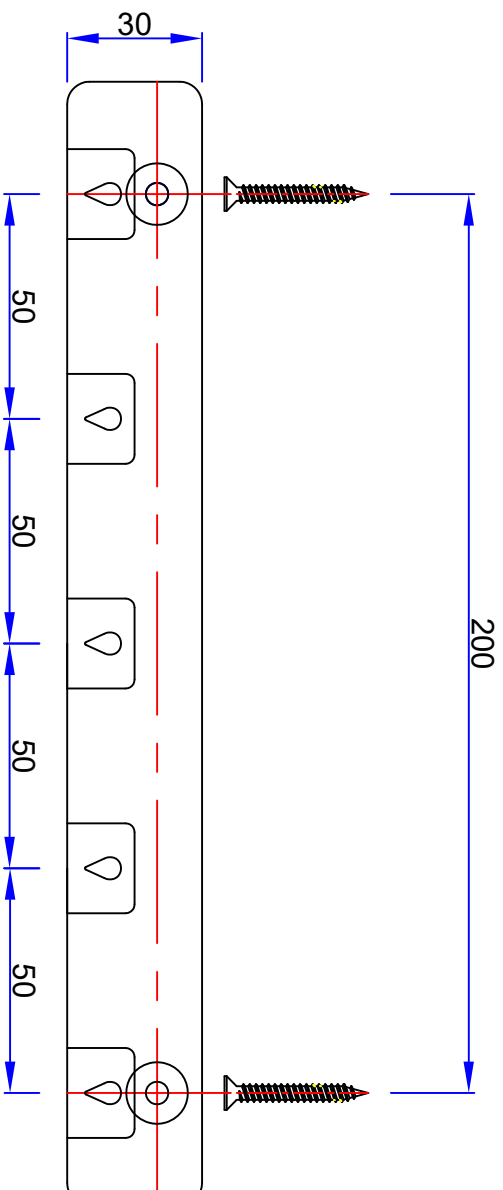
(Front View)
