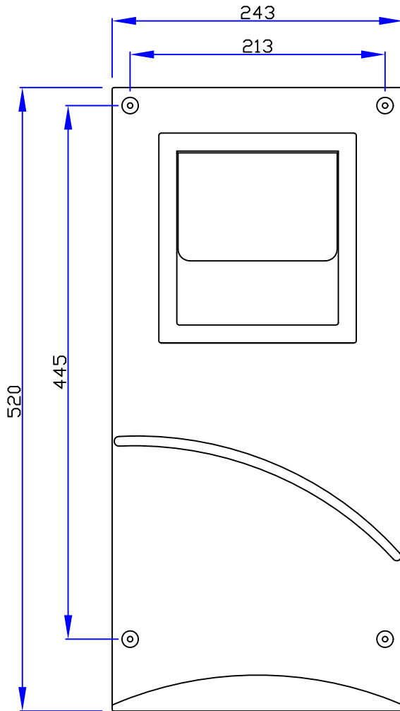
(Front View)
