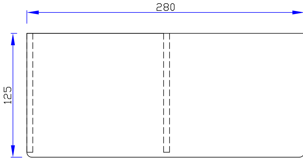
(Top View)
