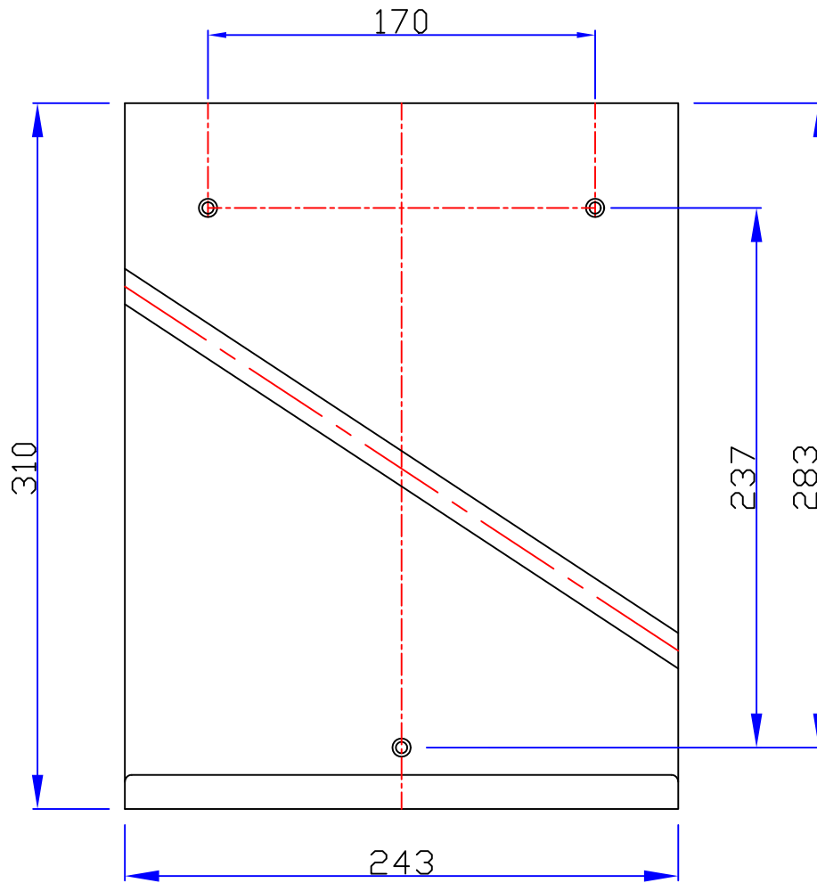
(Front View)
